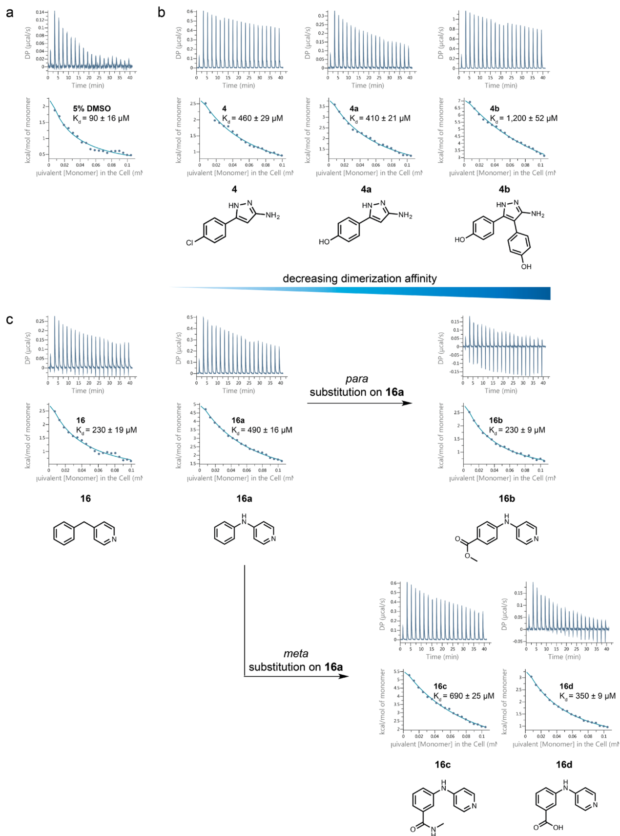
Figure 4. Thermally destabilizing fragments decreased the dimerization affinity in CK2 \beta P110D/V143D in homodissociation ITC experiments. (a) Homodissociation isotherm of CK2 \beta P110D/V143D in 5% (v/v) DMSO. (b) Homodissociation isotherms of 4 and its analogues ( 4a and 4b ). (c) Homodissociation isotherms of 16 and its analogues ( 16a–16d ). The top and bottom panels of each ITC profile illustrate the raw calorimetric data and the integrated heats per injection, respectively.
