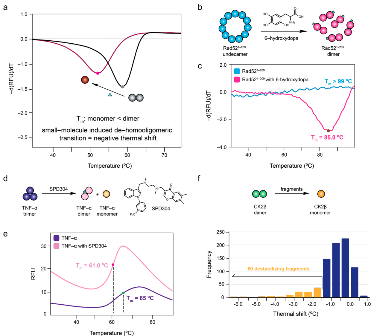
Figure 1. Use of fluorescence-based thermal shift assay to detect small molecules capable of inducing dehomooligomerization. (a) Hypothetical scheme illustrating whether small-molecule (triangle) disruption of a homodimeric assembly (black) to a monomeric state (red) is translated to a negative thermal shift. The first derivative of the melting curves are shown. (b) Schematic showing the undecameric-to-dimeric transition of Rad52 1-209 induced by 6-hydroxydopa (green). (c) Rad52 1-209 alone (blue) did not produce a melting transition, indicating that its T_m was more than 99 ^{\circ}\text{C} . In the presence of 6-hydroxydopa, Rad52 1-209 registered a T_m of 85.0 ^{\circ}\text{C} (red). (d) SPD304 (blue) causes the dissociation of native trimeric TNF- \alpha (purple) into a SPD304-bound dimer (pink) and monomer (yellow). (e) The melting curve of native trimeric TNF- \alpha (purple) showed that it had a putative T_m of 65 ^{\circ}\text{C} . In the presence of SPD304, the melting temperature of TNF- \alpha decreased to 61.0 ^{\circ}\text{C} (pink). (f) Distribution of thermal shift values induced by fragments in CK2 \beta from the fluorescence-based thermal shift screen.
